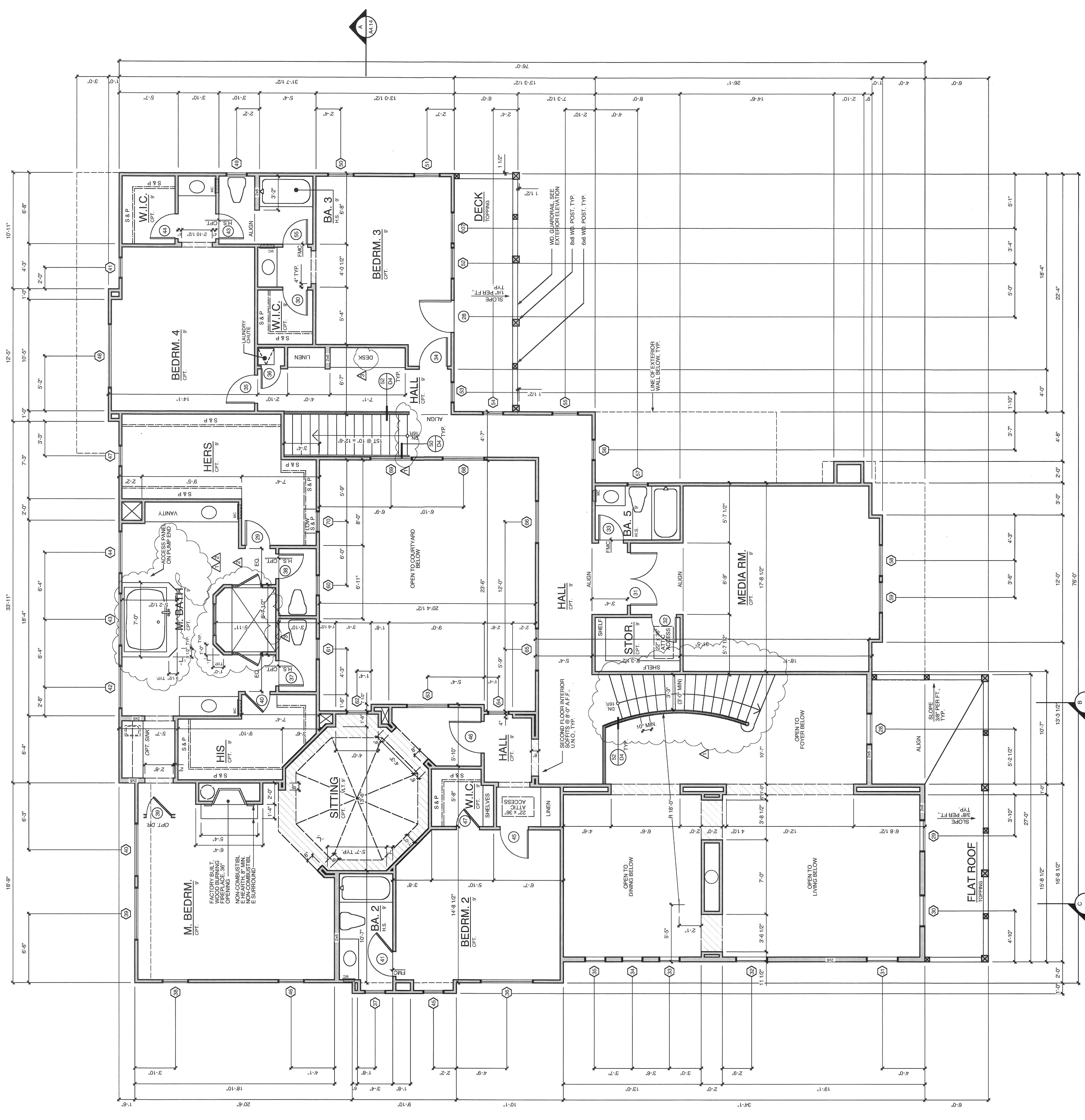
SECOND FLOOR PLAN 4A (COLONIAL REVIVAL) 1/4"=1'-0"
